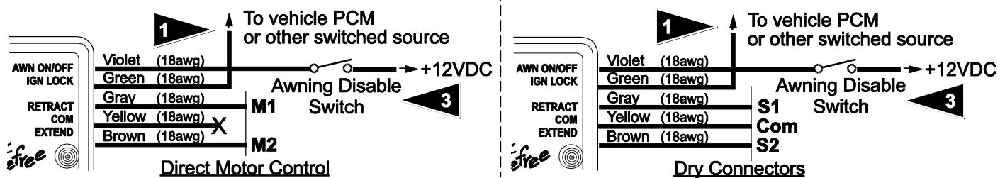
Single Pole, Single Throw Switch
