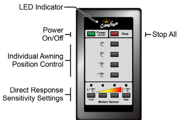
Single Awning
