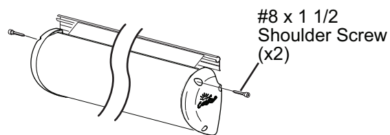
DETAIL C
