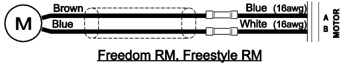
DETAIL A Motor Connect
