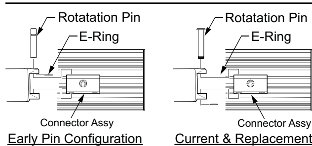
Detail A (Lead Rail Connector)
