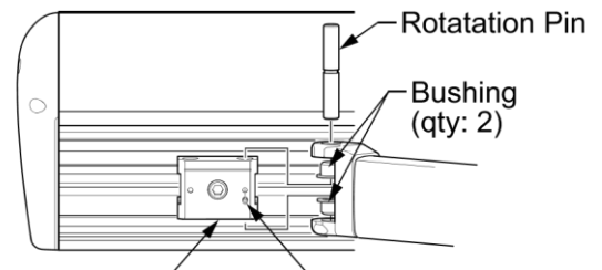
Connector Assy Detail B 6-32 x .25 set screw
