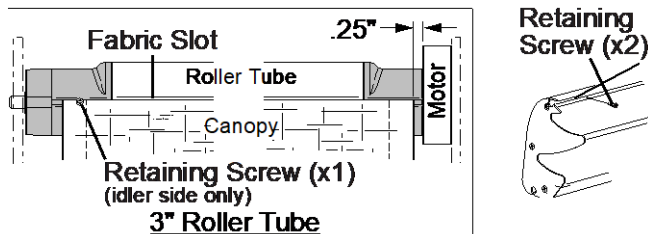
3" Roller Tube
