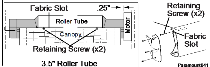
3.5" Roller Tube
