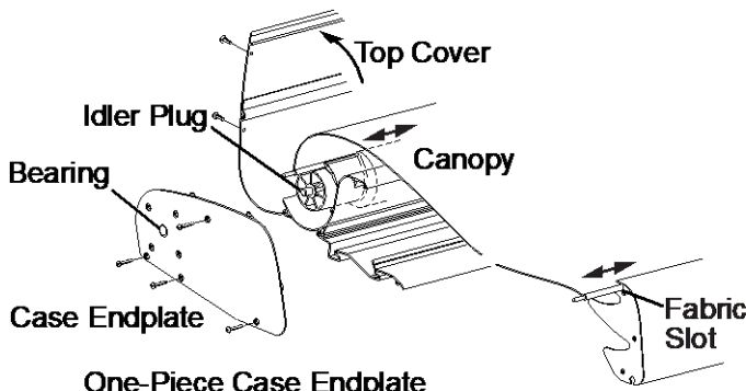
One-Piece Case Endplate
