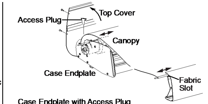
Case Endplate with Access Plug
