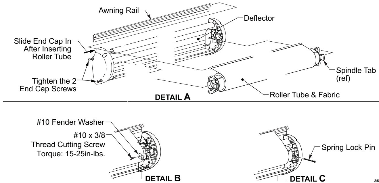
Figure 9. Installing the Roller tube Assembly.
