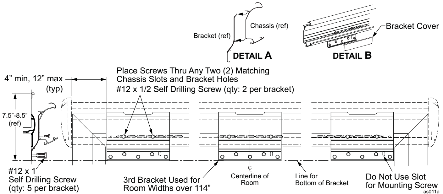
Figure 7. Mounting the Deflector w/ Brackets.
