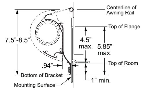
Figure 2. Direct Mount of Deflector.
