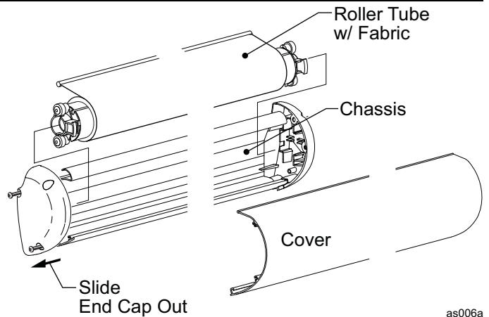
Figure 5. Unpacking the Unit.
