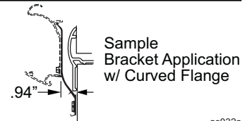
Figure 3. Deflector Mount w/ Bracket.
