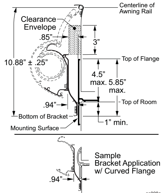
Figure 3. Deflector Mount w/ Bracket.
