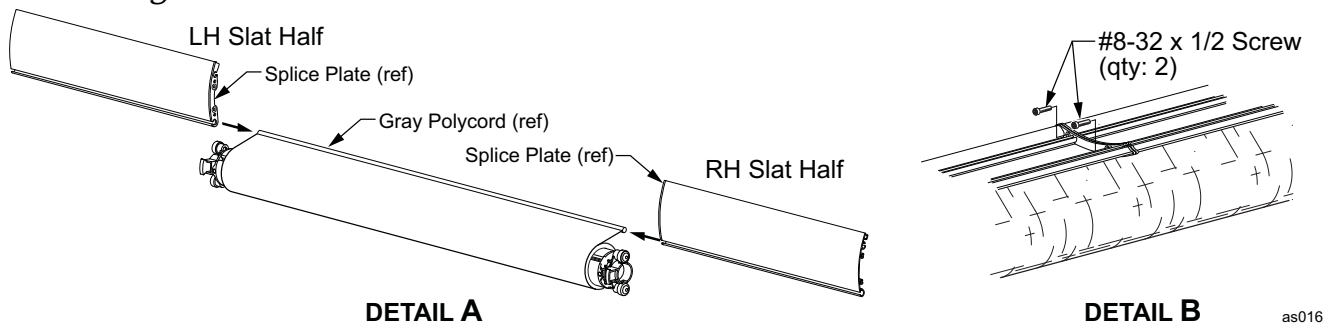
Figure 14. Mounting the Slat.
