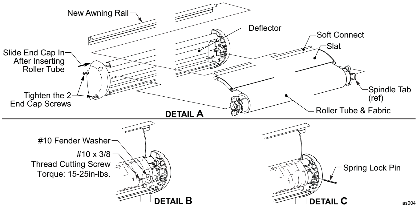
Figure 8. Installing the Roller tube Assembly.
