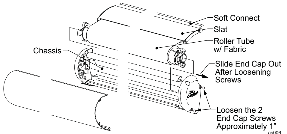
Figure 4. Unpacking the Unit.
