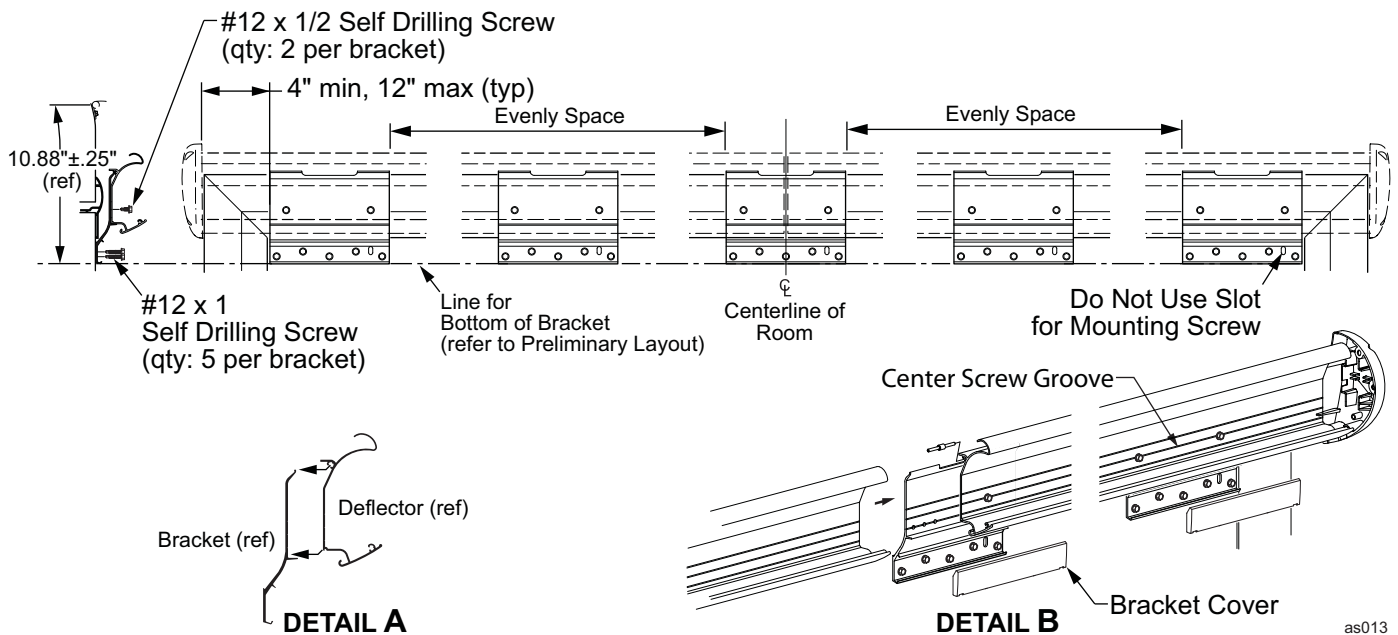
Figure 11. Mounting the Deflector w/ Brackets.
