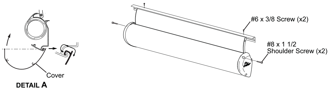
Figure 9. Installing the Cover.
