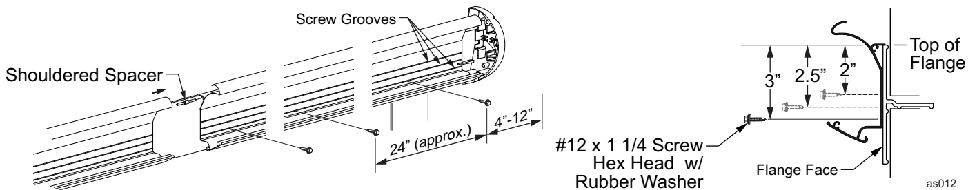
Figure 10. Installing the Deflector.
