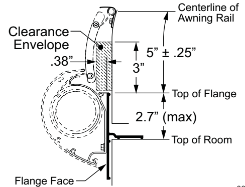
Figure 2. Direct Mount of Deflector.
