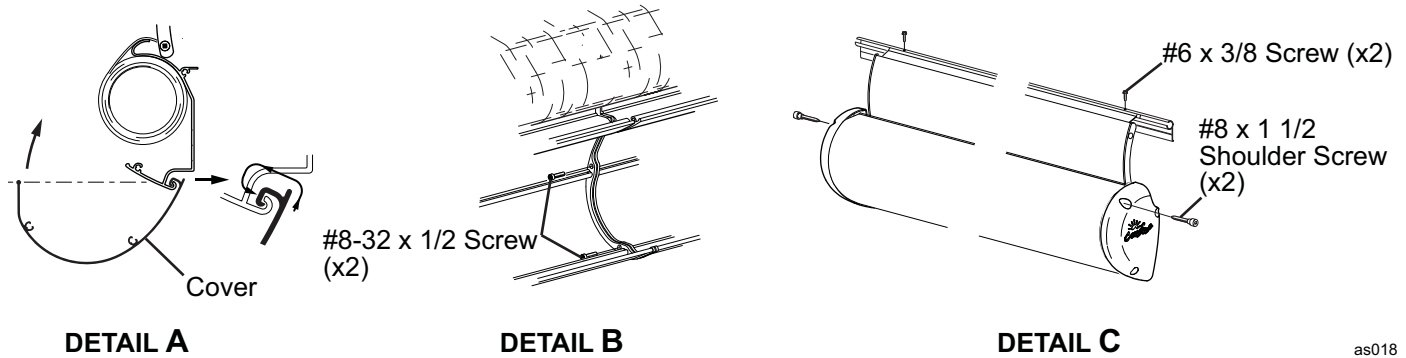
Figure 17. Installing the Cover.
