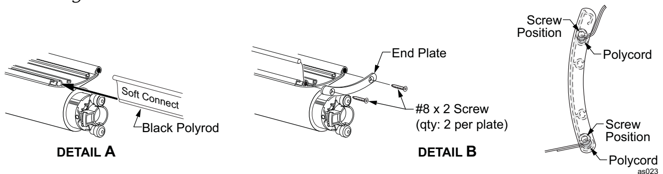
Figure 15. Inserting the Soft Connect.
