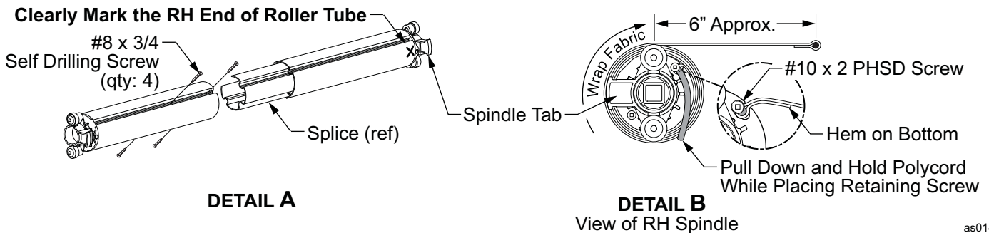
Figure 13. Assembling the Roller Tube.
