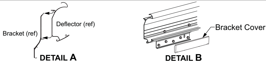
Figure 6. Mounting the Deflector w/ Brackets.
