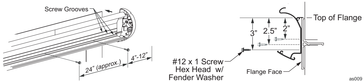
Figure 5. Installing the Deflector.
