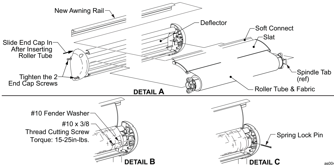
Figure 16. Mounting the Roller Tube Assembly.
